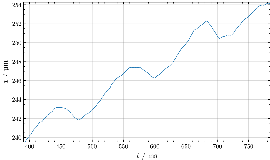
micromer-M (12.50 Hz, 20 ms): particle ID 7 (rank 8/14275)
